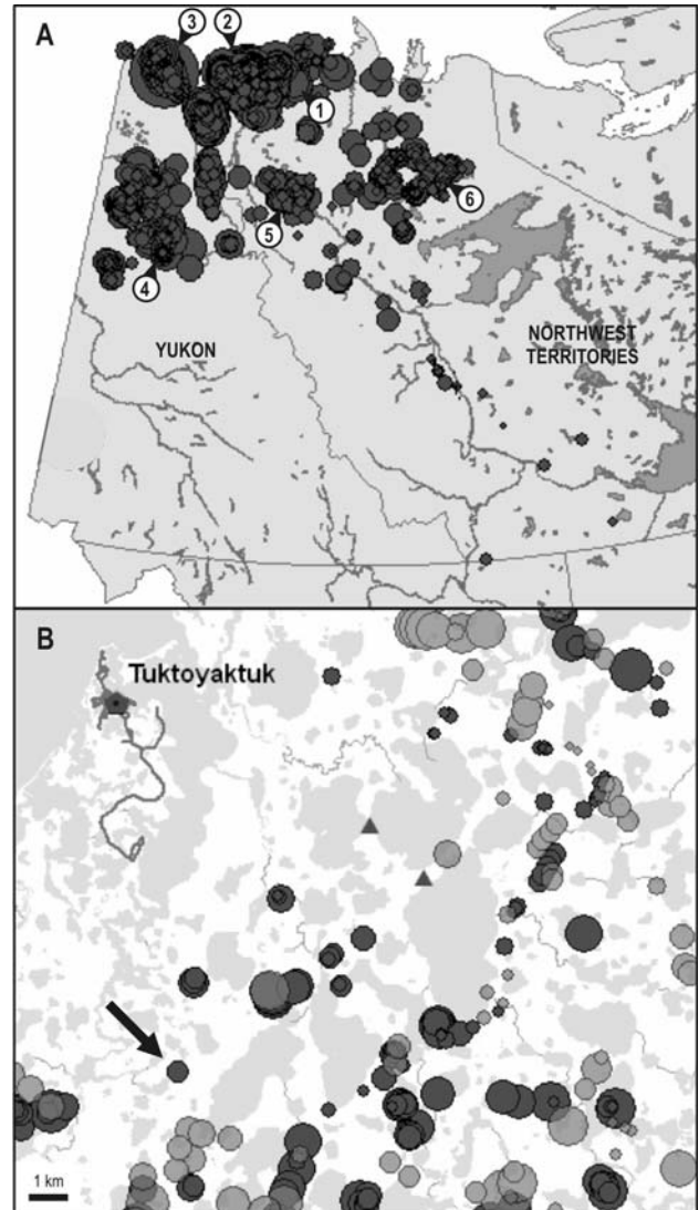
Figure 2. Massive ice records. A Distribution of shothole drillers' log records of massive ice represented by circular thickness-proportional symbols. Highest concentrations are found in the Tuktoyaktuk Peninsula – Richards Island – Beaufort coast areas (sites 1, 2, 3, respectively), with lesser occurrences in Eagle Plains (site 4), Little Chicago (northern Mackenzie corridor, site 5), and Colville Hills region (site 6). Few records are found in the central and southern Mackenzie corridor. B Detail of massive ice records southeast of Tuktoyaktuk, Northwest Territories. Dark circles are records derived from Smith and Lesk-Winfield (2010a); lighter circles are from Côté et al. (2003). Symbols illustrate thicknesses between 1 and 30 m; arrow points to a record interpreted to be 9.2 m thick (0-4.5 m, clay, rocks; 4.5-13.7 m, ice; 13.7-40 m, sand).
