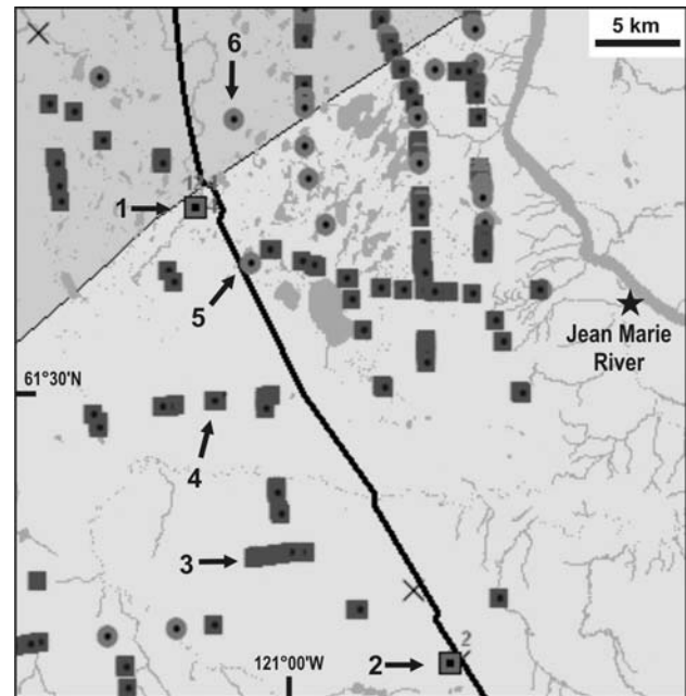
Figure 4. Seismic shothole drillers' log-derived estimates of minimum ice-bonded permafrost thicknesses in the Jean Marie River area, southern Northwest Territories. Squares represent sites with minimum estimates between 1-10 m; circles represent sites between 10-20 m. Numbered sites are referred to in the text. Dark, north-south oriented line is the path of the proposed Mackenzie Valley gas pipeline. Figure straddles the extensive discontinuous (dark shading) and sporadic discontinuous (lighter shading) permafrost zones.
