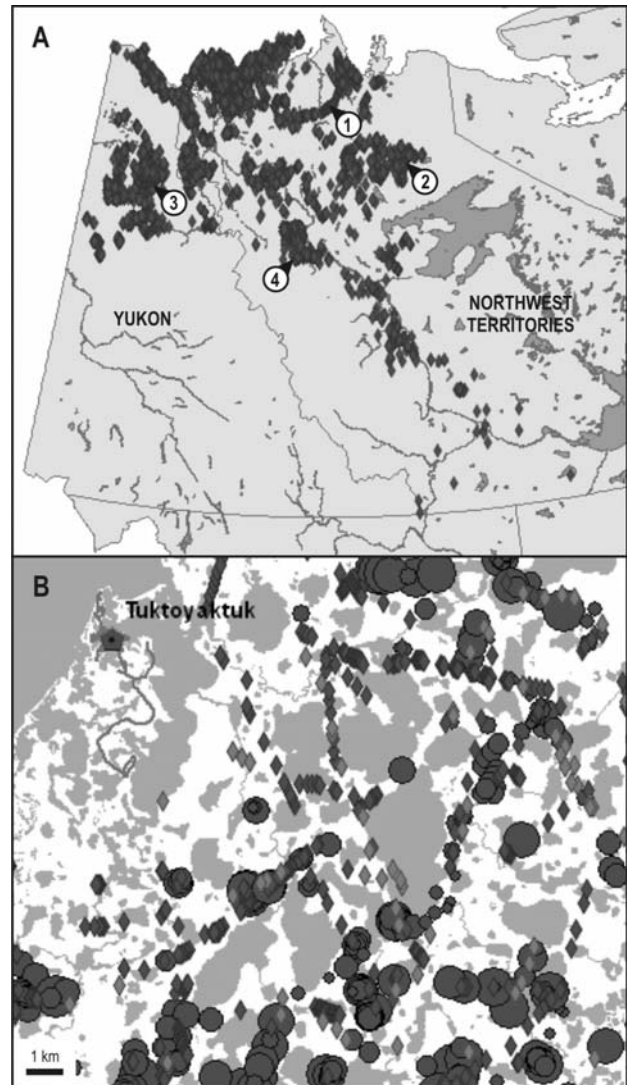
Figure 3. Ground Ice (thickness undefined) records. A Distribution of shothole drillers' log records of "ice" from compound sedimentary logs, represented by diamond symbols. Numbers refer to sites discussed in the text: Anderson River (1), Colville Hills (2), Eagle Plain (3), Ramparts River (4). B Detail of "ice" records southeast of Tuktoyaktuk, Northwest Territories, along with massive ice records (Fig. 2B). Dark diamond symbols are ground ice records derived from Smith and Lesk-Winfield (2010a), lighter diamond symbols are ground ice records from Côté et al. (2003).
