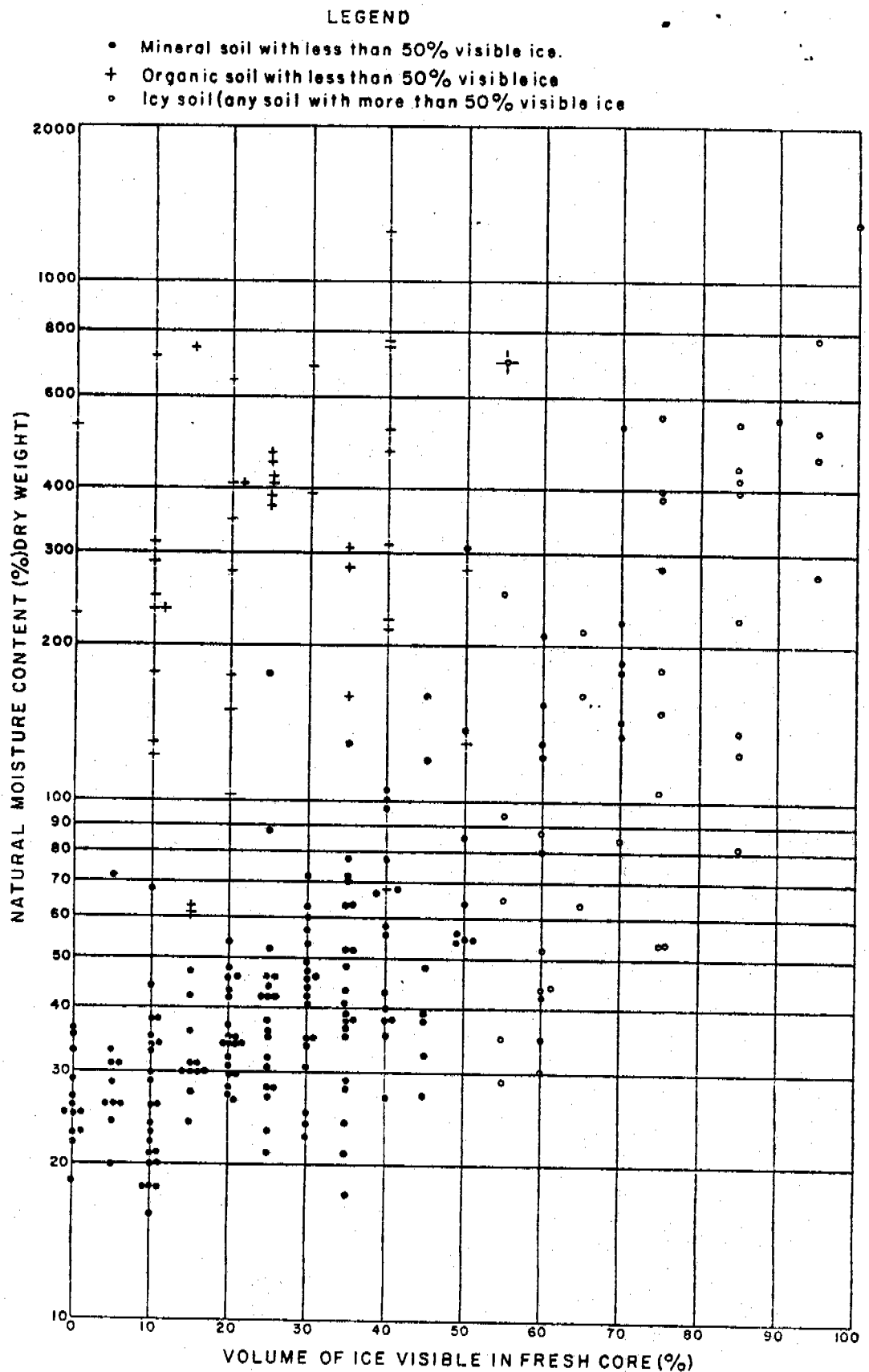
Figure 7. Relationship between visible ice content and natural water content
